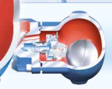
CONA® SC PN 40 with outside strainer (Y) Compact and lightweight due to the slim design
