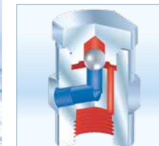
Vacuum breaker
