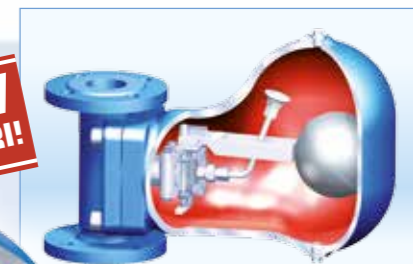
Extra-high performance version for condensate volumes > 10,000 kg/h and differential pressures up to 32 bar. Robust lever and ball design
